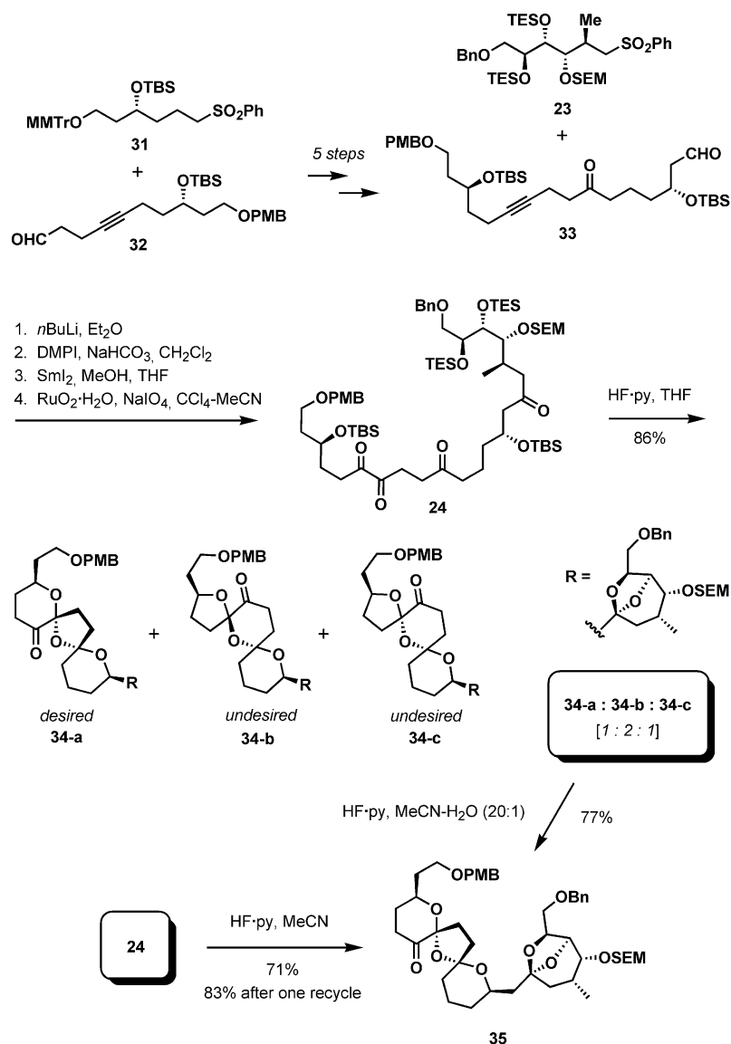
Scheme 7. Synthesis of the BCDEF ring.
