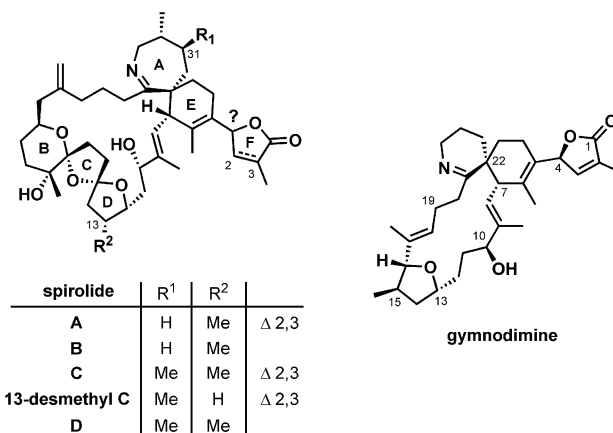
Figure 3. Spiroimine marine toxins: spiroolides A–D and gymnodimine.
