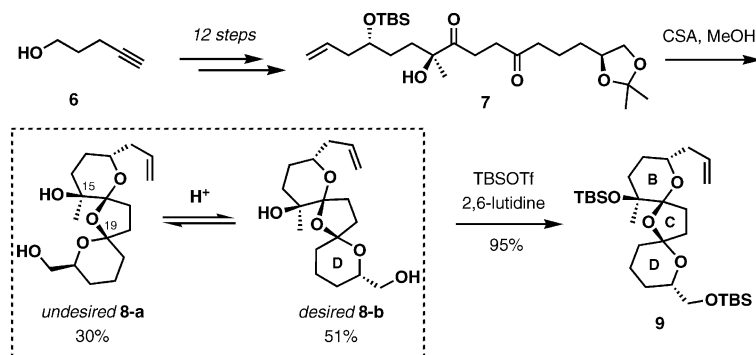
Scheme 2. Synthesis of the BCD-spiroketal.
