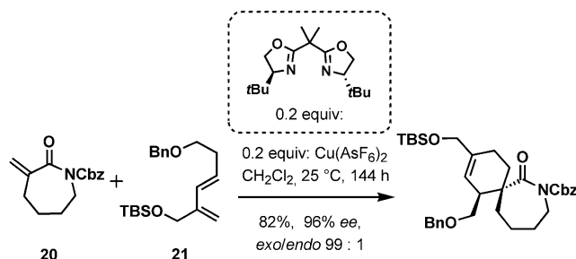
Scheme 8. Diastereoselective formation of the spiroimine ring through a copper-bisoxazoline-catalyzed Diels–Alder reaction.
