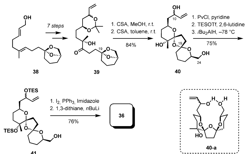
Scheme 10. Preparation of the BCD ring.
