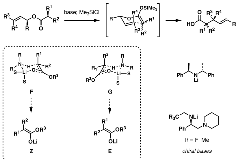
Figure 4. Transition structures of the Ireland–Claisen rearrangement.
