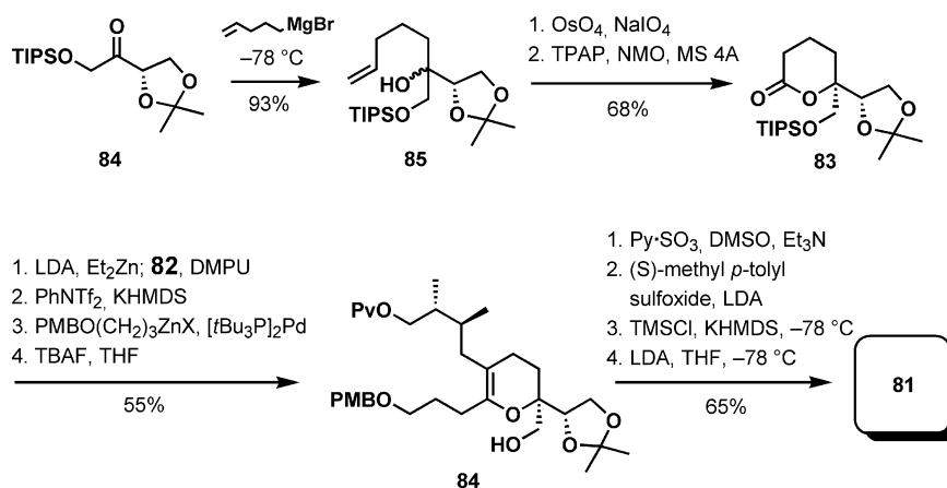
Scheme 18. Synthesis of the vinyl sulfoxide 81 .
