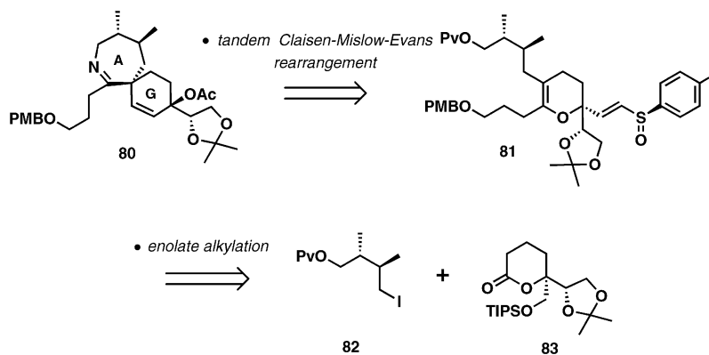
Scheme 17. Initial approach to the AG-spiroamine ring.
