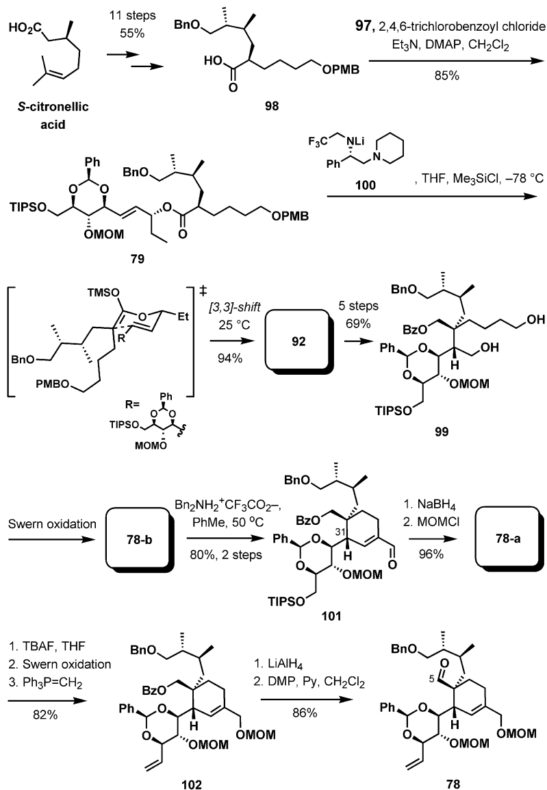
Scheme 24. Application of the [3,3] sigmatropic shift.
