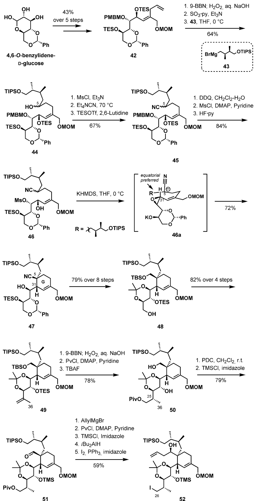
Scheme 11. Synthesis of fragment 52.
