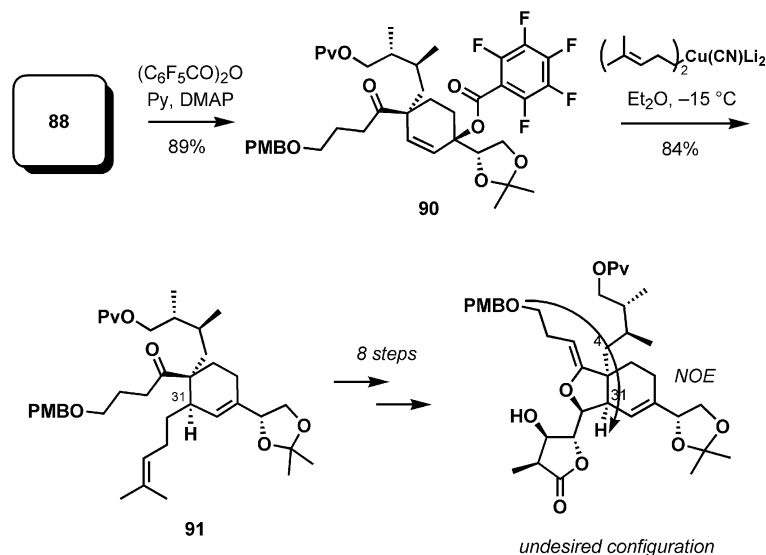
Scheme 19. Cascade Claisen–Mislow–Evans rearrangement.
