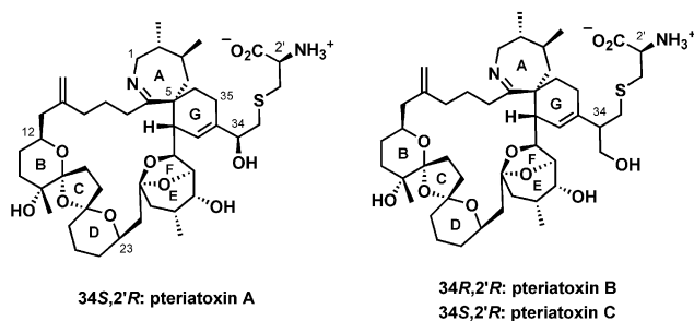
Figure 2. Spiroimine marine toxins: pteriatoxins A–C.
