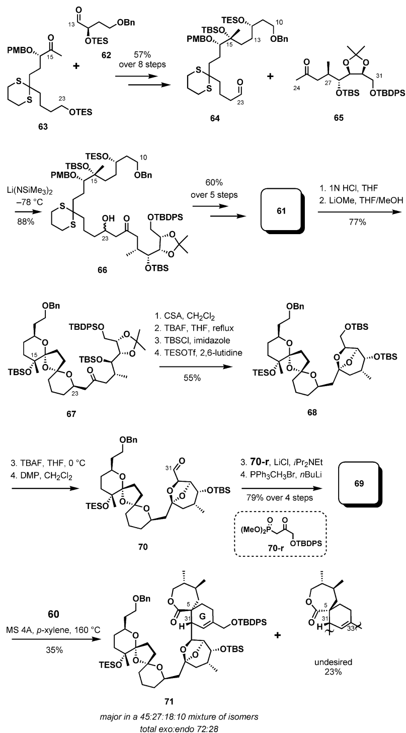
Scheme 14. Synthesis of the Diels–Alder adduct.
