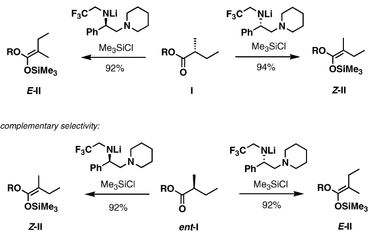
Scheme 22. Chirality of the base dictates stereoselectivity.
