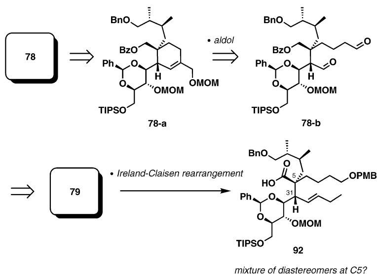
Scheme 21. New strategy for spiroamine formation.
