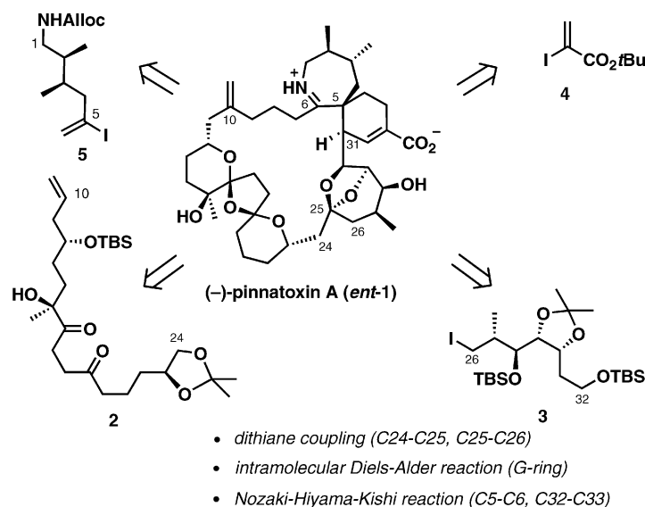
Scheme 1. Synthesis plan for (–)-pinnatoxin A.
