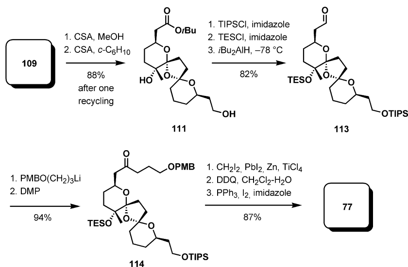
Scheme 26. Completion of fragment 77 .
