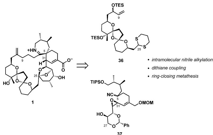
Scheme 9. Synthetic strategy for (+)-pinnatoxin A ( 1 ).
