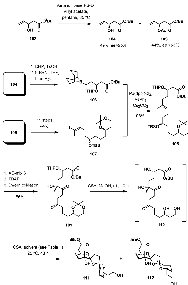
Scheme 25. Preparation of the BCD-spiroketal precursor.
