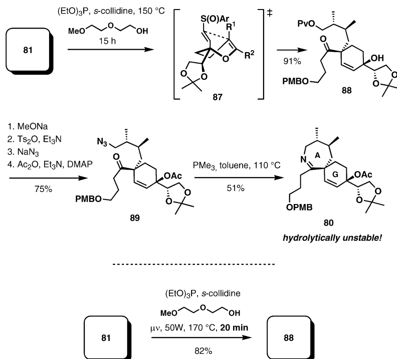
Scheme 19. Cascade Claisen–Mislow–Evans rearrangement.
