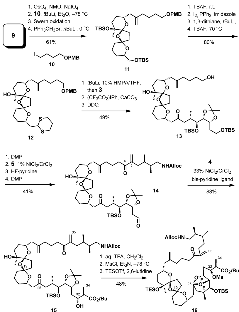
Scheme 3. Synthesis of the substrate for the intramolecular Diels–Alder reaction.
