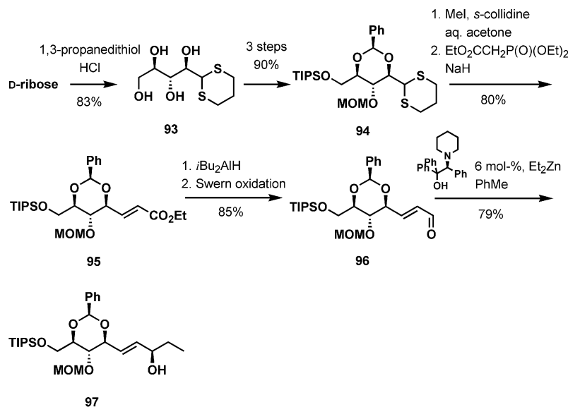
Scheme 23. Preparation of the allylic alcohol 97.
